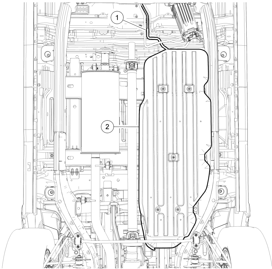
Fuel Tank — Bottom View, Long Wheelbase
