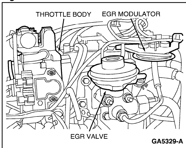
Figure 5: EGR Valve
