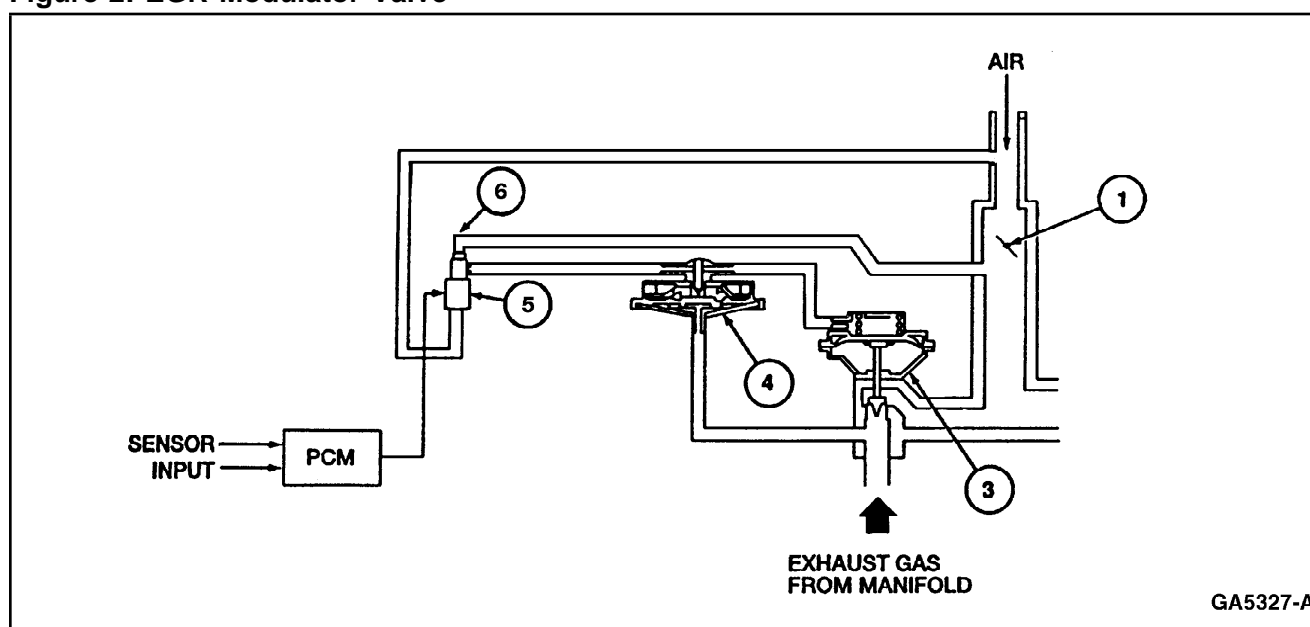
Figure 2: EGR Modulator Valve
