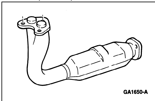
Figure 3: Warm Up Three Way Catalytic Converter (WU-TWC) Converter
