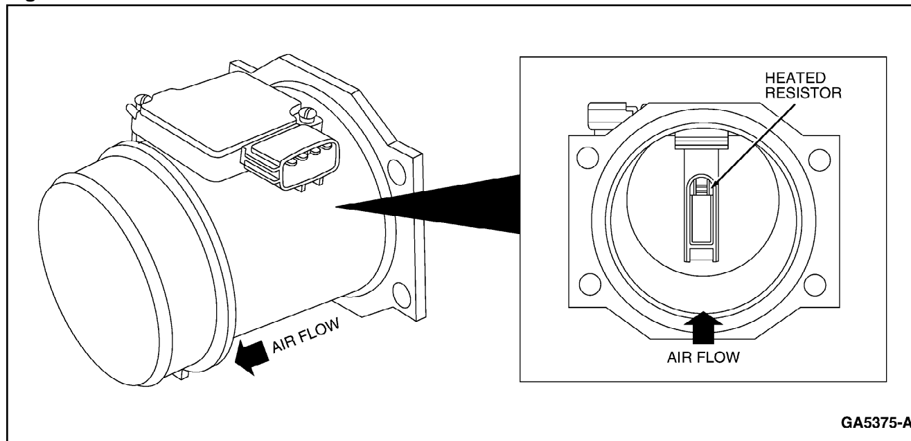
Figure 4: MAF Sensor
