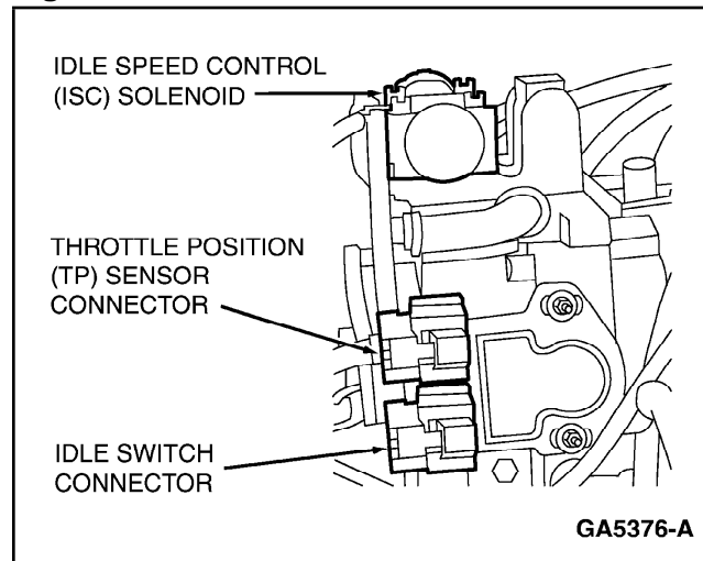
Figure 6: TP Sensor
