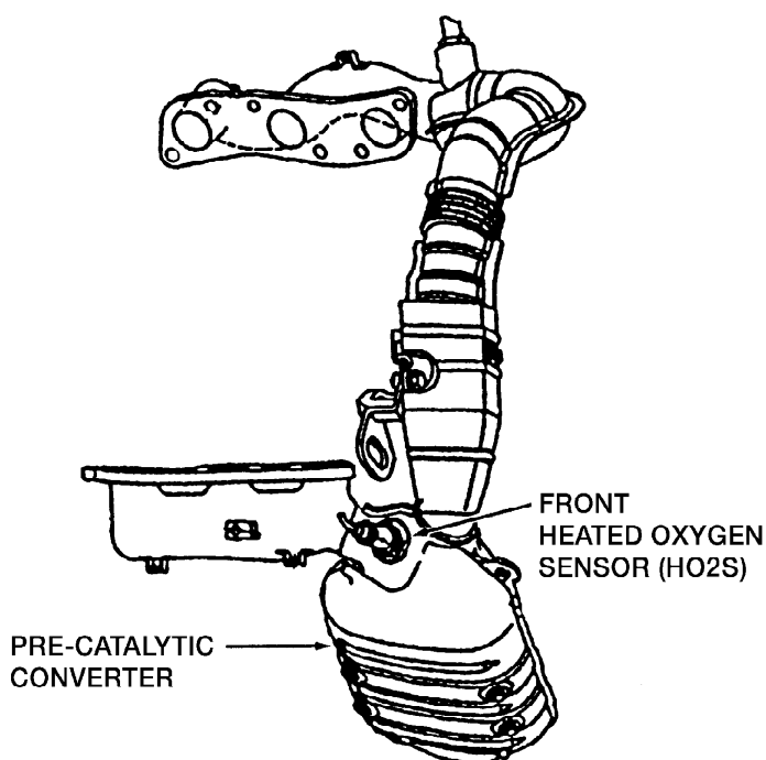
Figure 4: Pre-Catalytic Converter
