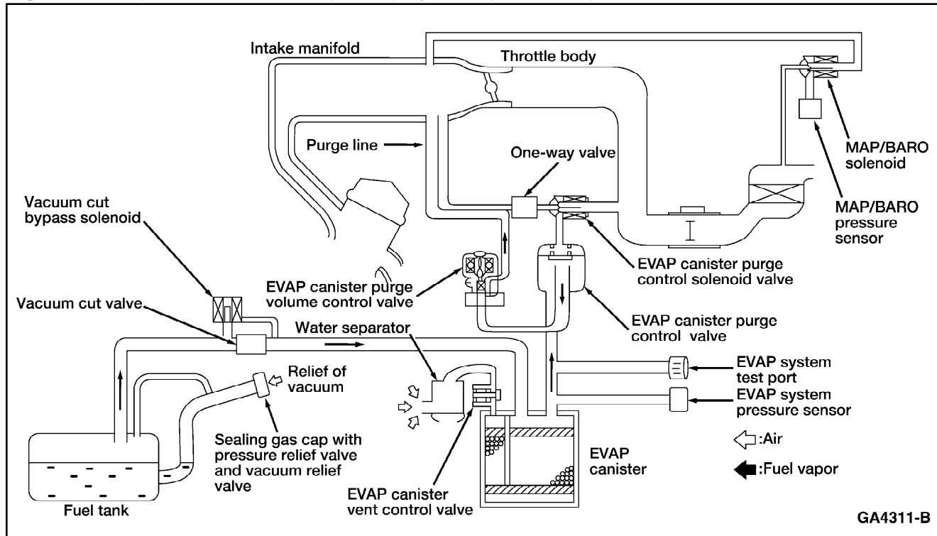
Figure 5: Evaporative Emission (EVAP) System (California)
