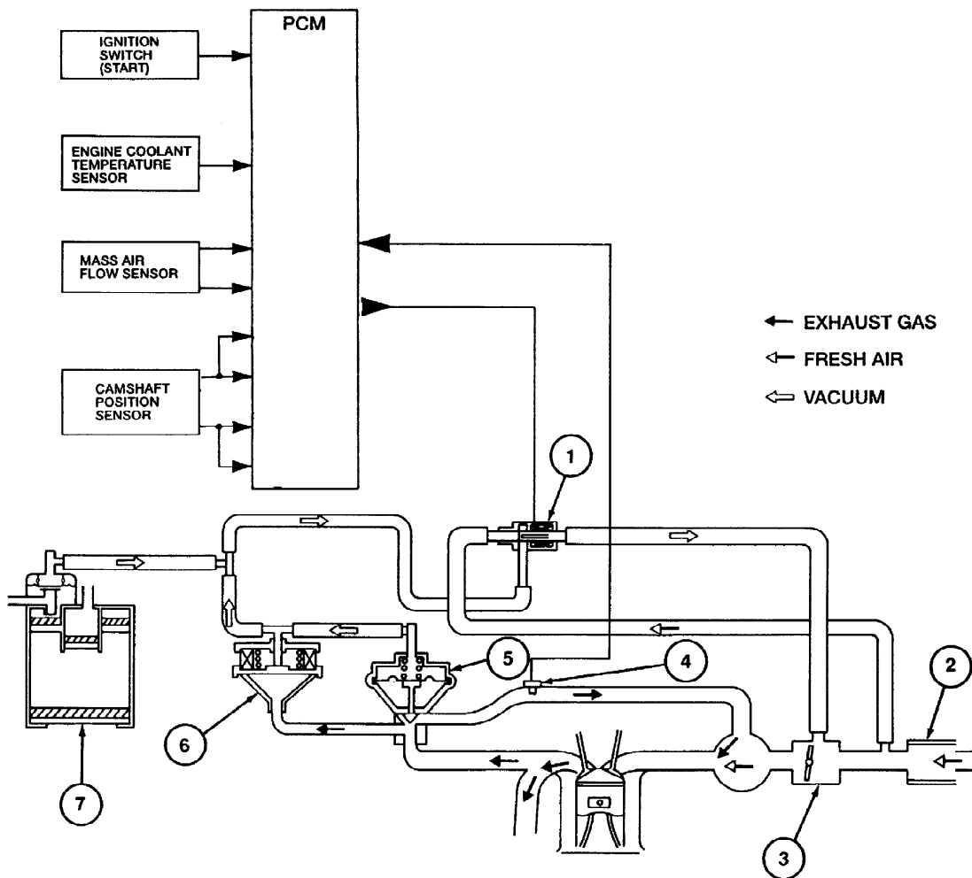
Figure 1: Exhaust Gas Recirculation (EGR) System Diagram (Federal Emissions)
