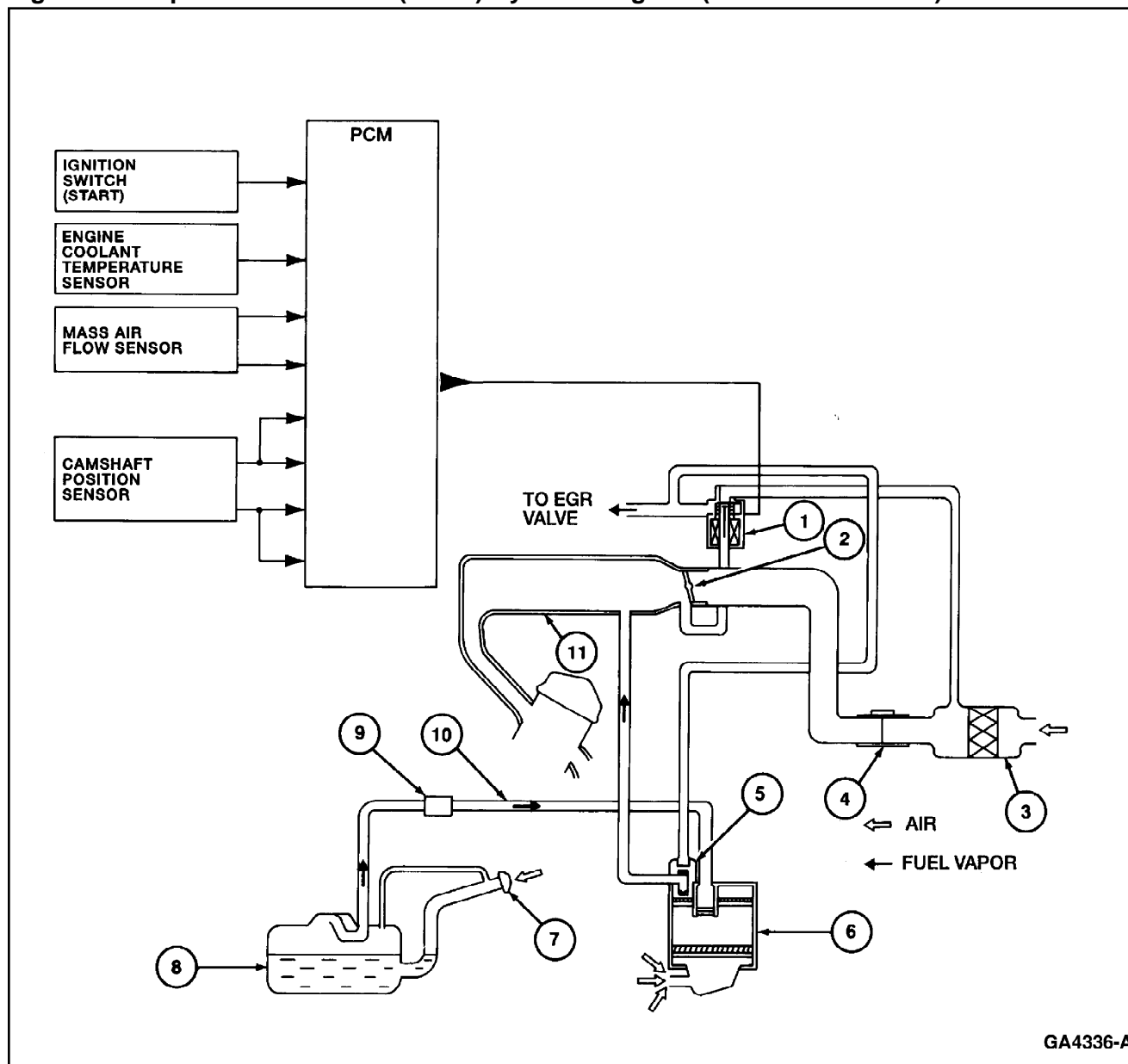
Figure 1: Evaporative Emission (EVAP) System Diagram (Federal Emissions)
