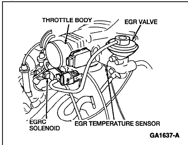
Figure 6: EGR Valve
