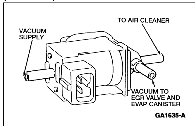
Figure 4: Exhaust Gas Recirculation/Evaporative Emission (EGR/EVAP) Control Solenoid
