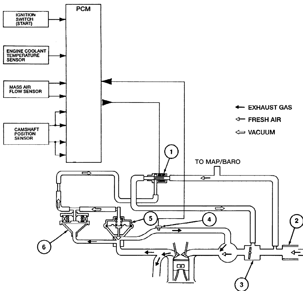
Figure 2: Exhaust Gas Recirculation (EGR) System Diagram (California Emissions)
